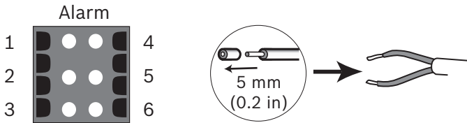
Figure 5.6 Alarm and relay connector pins
